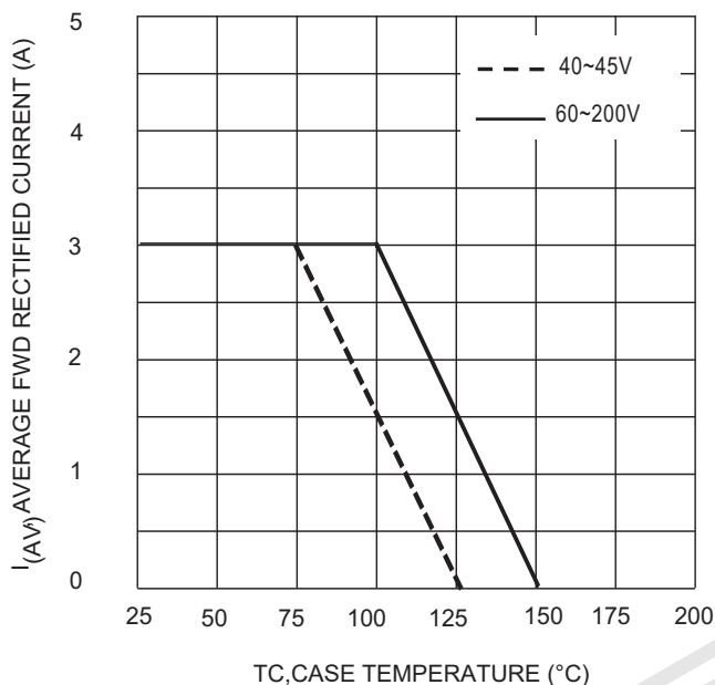
TC,CASE TEMPERATURE ( ^{\circ}\text{C} ) Fig. 1 Forward Derating Curve
