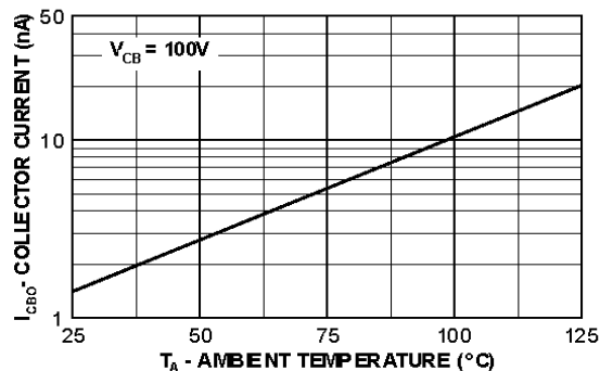
Collector-Cutoff Current vs. Ambient Temperature
