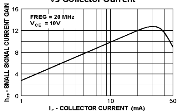
Small Signal Current Gain vs Collector Current
