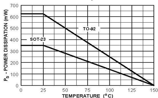
Power Dissipation vs Ambient Temperature
