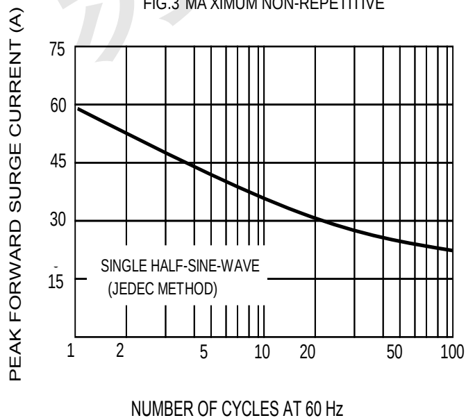
FIG.3 MAXIMUM NON-REPETITIVE
