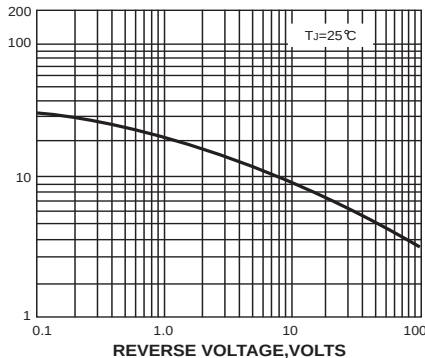
FIG. 5-TYPICAL JUNCTION CAPACITANCE
