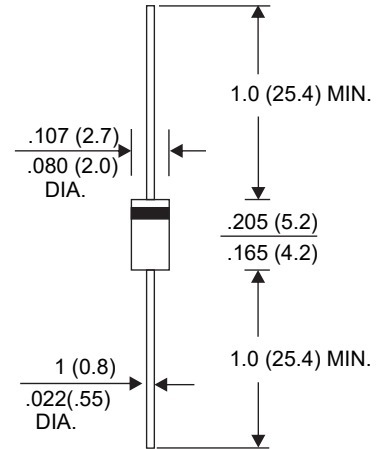
DO-41(DO-204AL)
